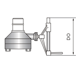
Yoke For NPS10 & Larger
